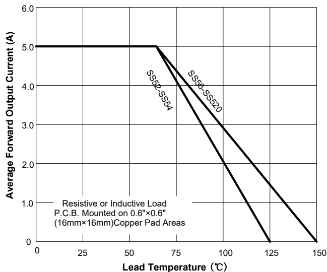
FIG.1: Io-Ta Curve
